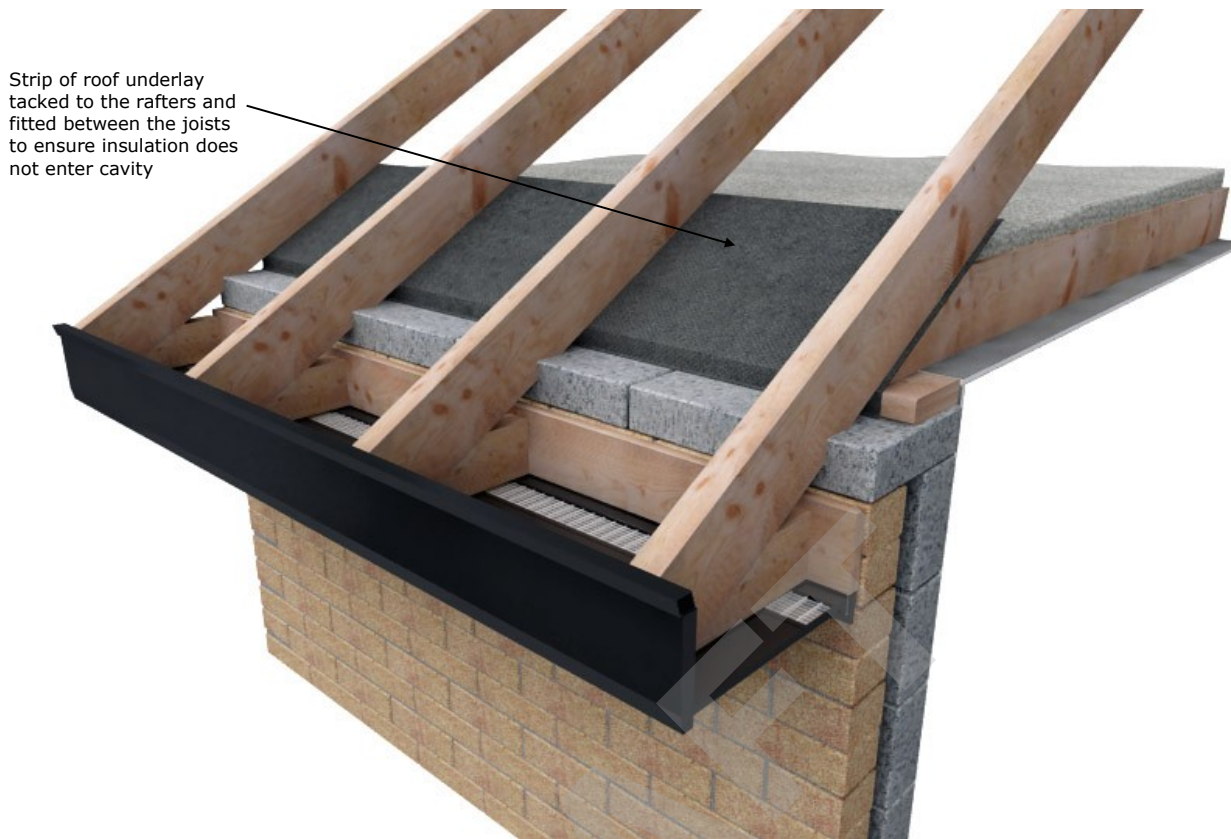
Figure 3: Eaves Detail
