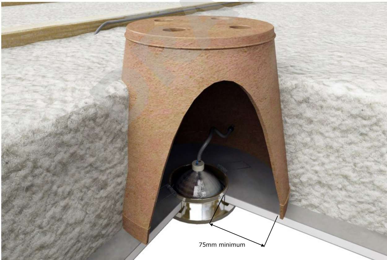
Figure 2: Light Guard Detail
